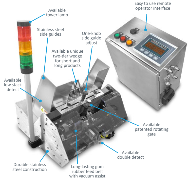
Shown with dual hopper configuration
